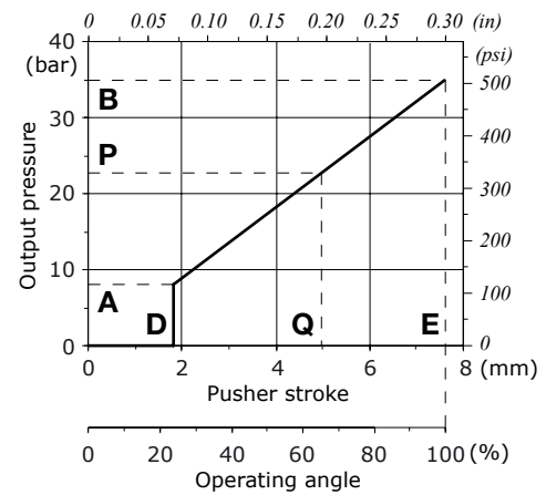
E1 type with pre-feeding for EM detent
