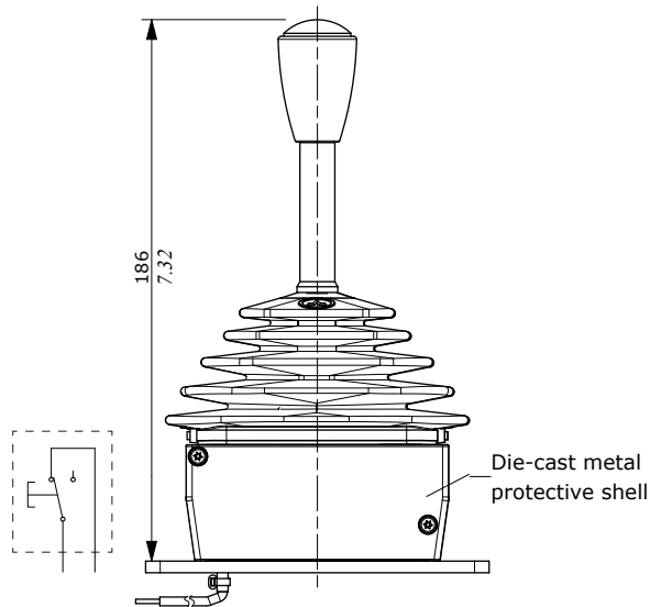
16TM3G3(NC)-16TM1G3(NC)-16TM2G3(NC) control
