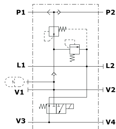
Hydraulic circuit
