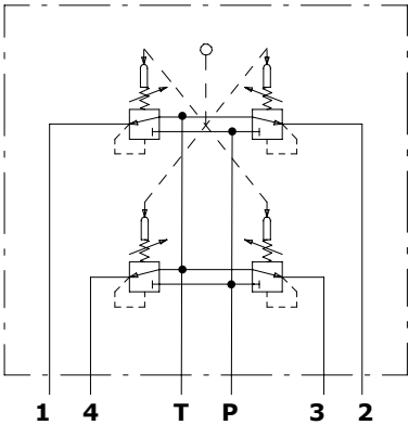
Hydraulic circuit
