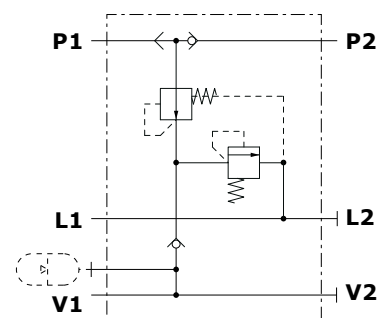
Hydraulic circuit
